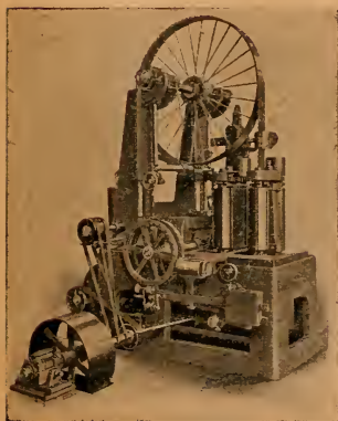
"Berlin" Line Wood-Working Machinery
