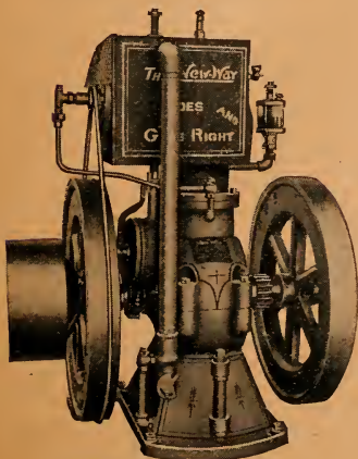
"New Way" Air-Cooled Otto Gasoline Engines
